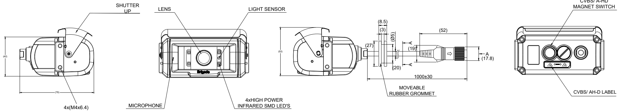
VIEW A
